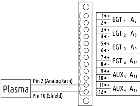
Figure 33: Connection of Plasma RPM analogue voltage output signal to A channel.
