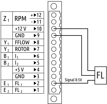
Figure 30: An example of capacitive fuel level probe connected to the +12 V power source. Some probes require 5 V, be careful.
