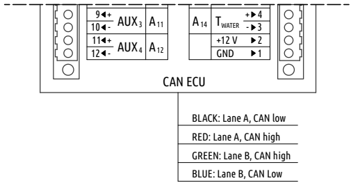
Figure 40: Color codes of the 4-pin connector. Two lanes can be connected, each has two wires. Some engines connect only one lane. WMFly Engine - CCM module, for example.
