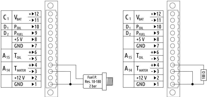
Figure 41: Example: VDO 2 bar sensor was replaced by a fixed 100 Ohm resistor.
