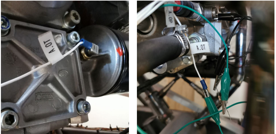
Figure 42: Test setup. Left: Location of the oil temperature sensor and its lead to Daqu (labeled as A.OT). Right: Oil temperature lead was detached and connected with green cable to one side of the test resistor. The other side of the resistor connects to an appropriate engine point (black cable).
