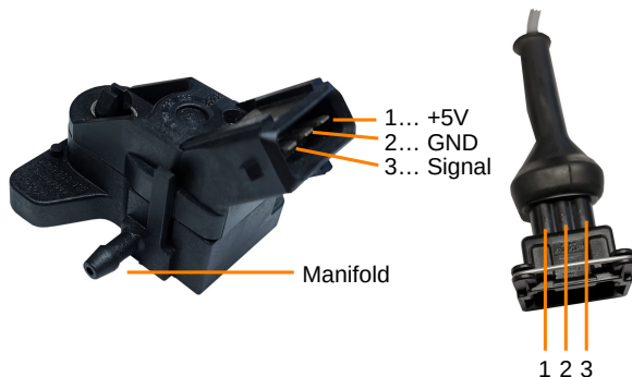
Figure 34: External manifold pressure sensor, Bosch 0 261 230 037.
