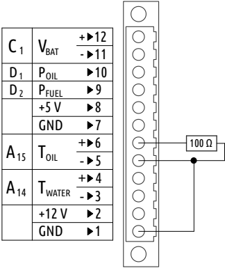
Figure 43: Example: VDO oil temperature sensor was replaced by a known test resistor. A 100 Ω resistor is shown, but any other test resistor from Table 36 can be also used.
