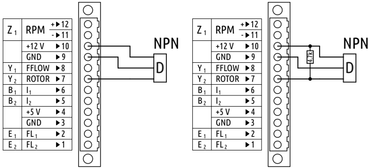
Figure 13: Left: a typical example of NPN digital sensor connection. Right: In some cases an external 4.7\text{ k}\Omega pullup resistor is needed.
