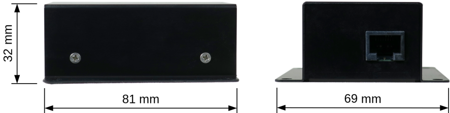
Figure 1: Front and side view of the UPSL with its principal dimensions.
