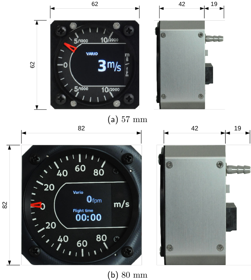
Figure 1: Front and side view of the variometer with its principal dimensions.
